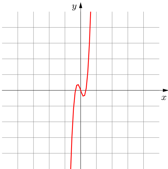
f(ax) Stretched Horizontally ( \leftrightarrow ), scale factor \frac{1}{a}
