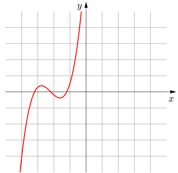
f(x + a) Moved Left ( \leftarrow ) by a units
