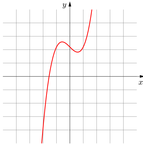
f(x) + a Moved Upwards ( \uparrow ) by a units
