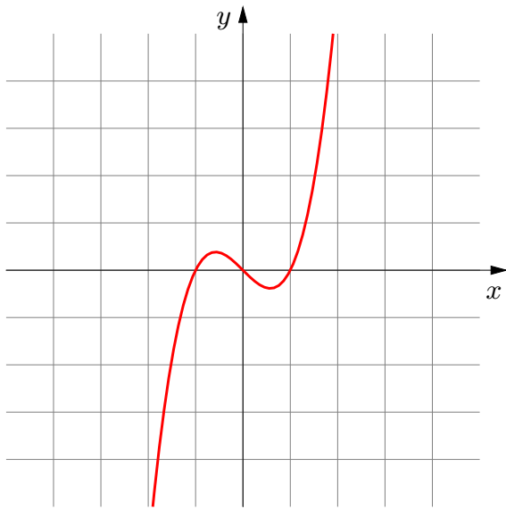
f(x) Original Function
