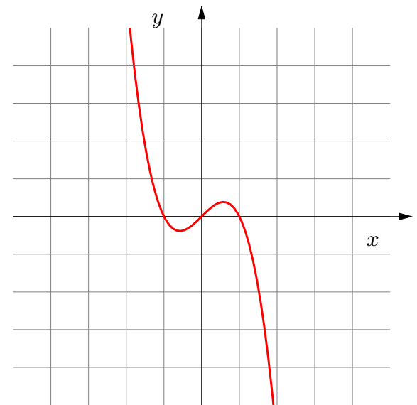
-f(x) Reflected in the x -axis
