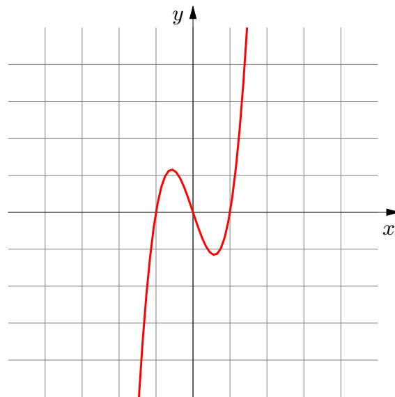
af(x) Stretched Vertically ( \updownarrow ), scale factor a
